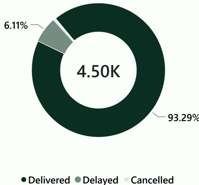
Order Outcomes
